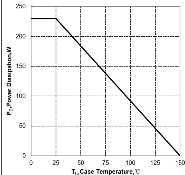
Figure 2a Power Dissipation (TO-220/TO-263)
