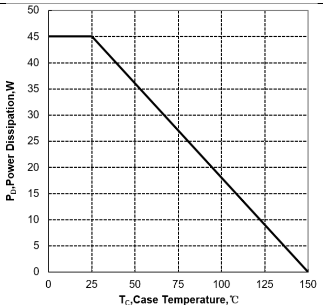
Figure 2b Power Dissipation (TO-220F)
