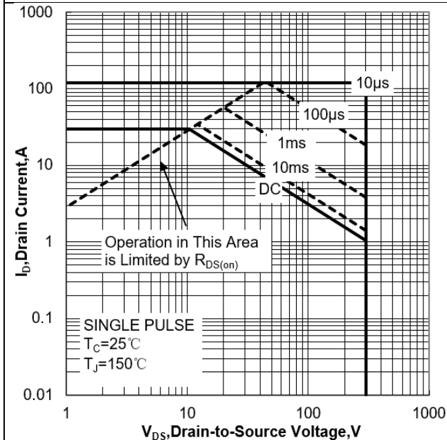
Figure 1a Safe Operating Area (TO-220/TO-263)
