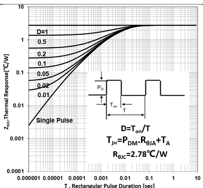
Figure 3b Max Thermal Impendence (TO-220F)
