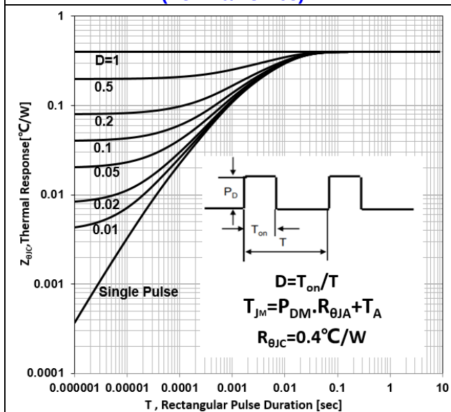
Figure 3a Max Thermal Impendence (TO-220/TO-263)
